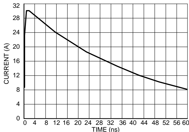
Figure 7. IEC 61000–4–2 ESD Test Waveform ( V_S = 8.0 kV, R = 330 \Omega , C = 150 pF)
