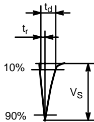
Figure 12. ISO 7637-3 Test Pulse 'a'
