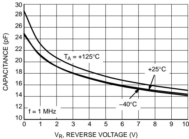
Figure 6. Capacitance versus V_R Characteristic of the NUP2105L
